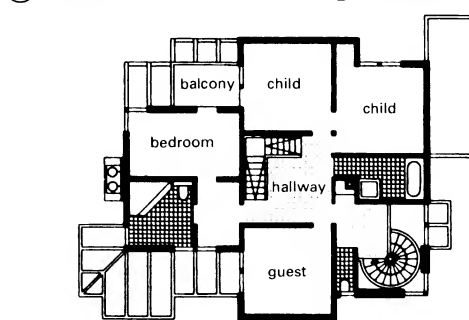
11 Top floor
